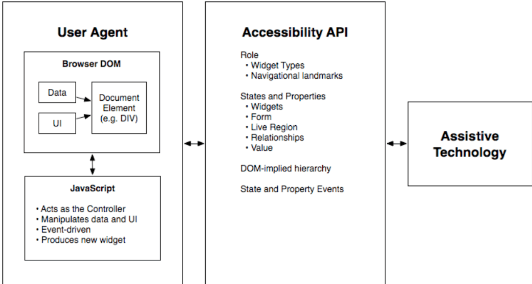
Figure 1: The contract model with accessibility APIs
